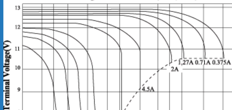
Discharge Characteristics (20°C, 68°F)
