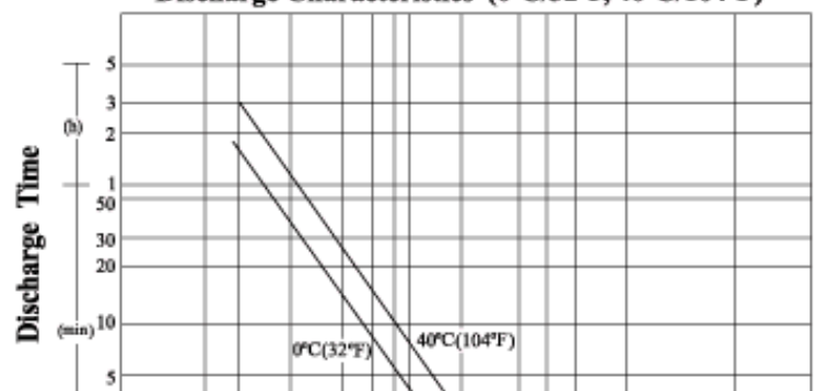
Discharge Characteristics (0°C/32°F, 40°C/104°F)
